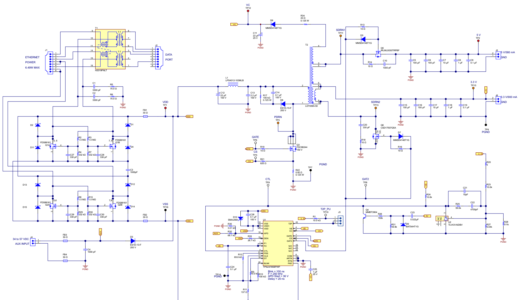
Figure 1. TPS23785BEVM-522 Schematic
